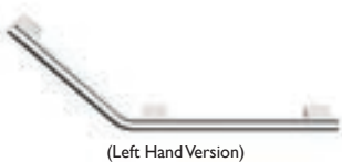
Design Line Angled Grab Bar 670 x 90 x 240 mm
