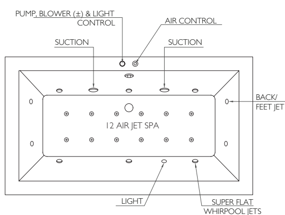
System 6ESF - Super Deluxe SPA 6 Self-Cleaning Super Flat Whirlpool Jets, Electronic Control Switch, 2 Back & 2 Feet Jets, Underwater Lighting, 12 Spa Air Jets on Bath Tub Base
